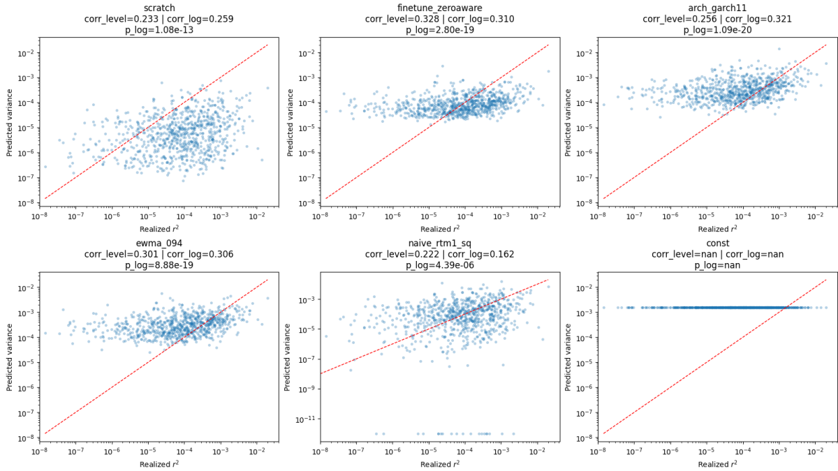
Figure 3: Predicted variance versus realized r^2 on the filtered real-data evaluation sample. The zero-aware finetuned model forms the tightest cloud among the neural methods and substantially improves over scratch training.
