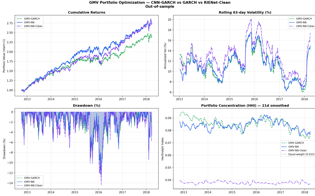
Figure 5: Example cumulative comparison from the constrained GMV experiments.
