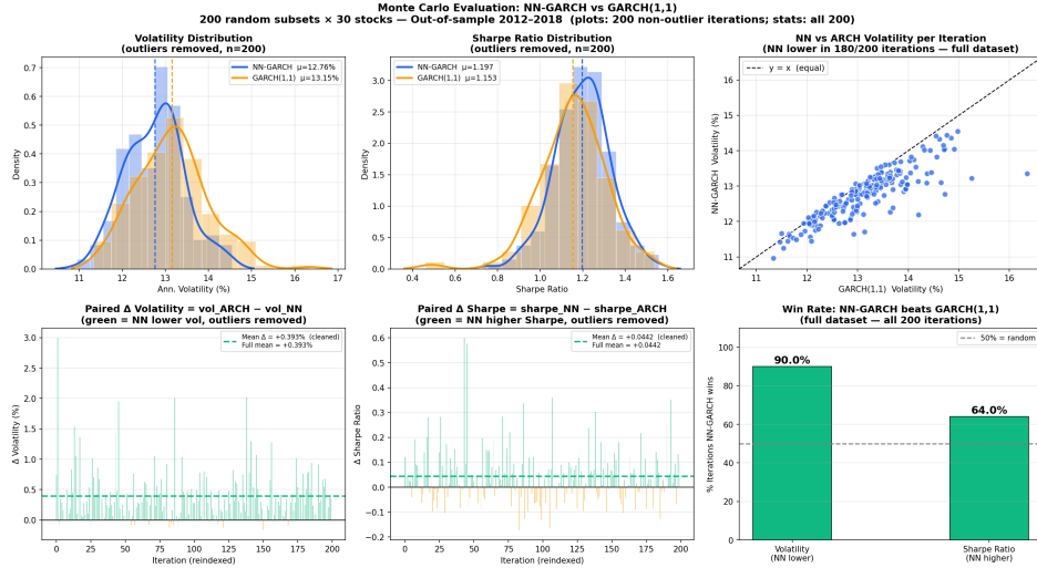
Figure 6: Monte Carlo distributions used for the paired Wilcoxon robustness study.
