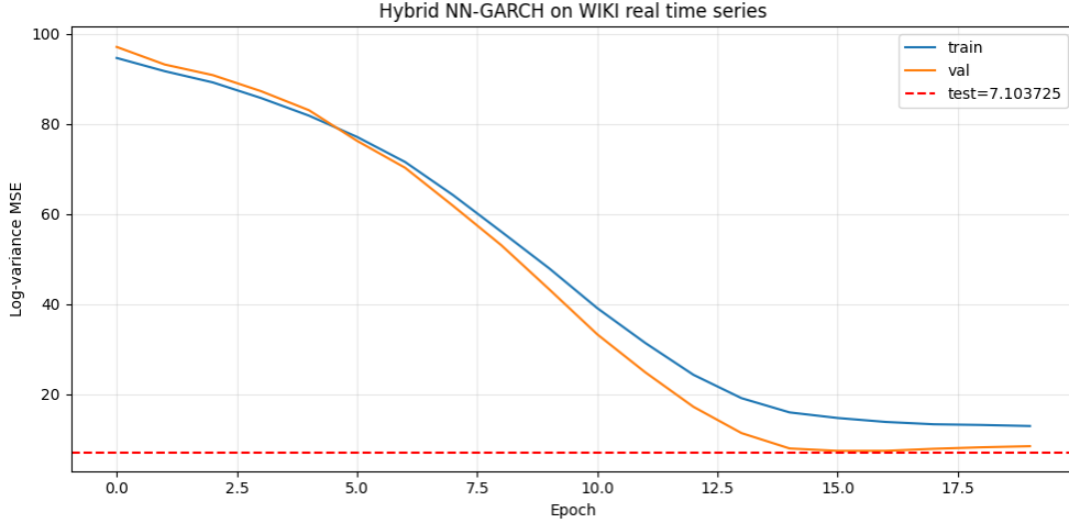
Figure 2: Example real-data training curve for the hybrid NN-GARCH model on WIKI returns. The gap between train and validation remains controlled while both losses decrease sharply over the first fifteen epochs.
