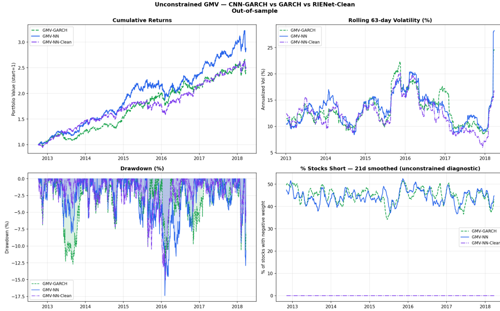
Figure 4: Cumulative performance comparison for the 50-stock unconstrained GMV experiment.
