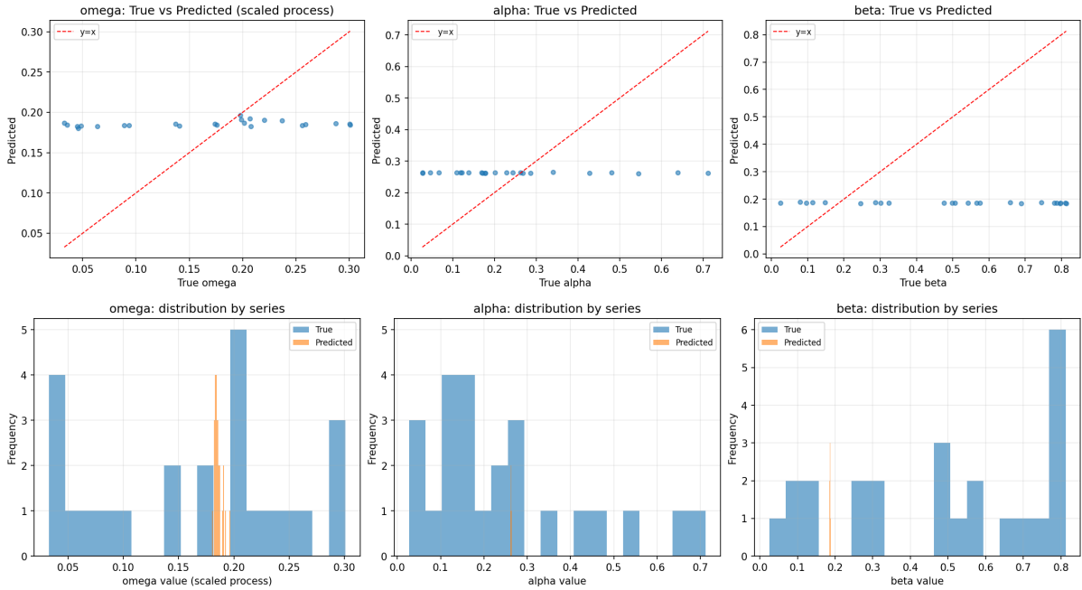
Figure 1: Synthetic pretraining diagnostics on simulated GARCH(1,1) series. Top: per-series true versus predicted parameters. Bottom: distribution of true and predicted parameters after scaling the process by the training standard deviation.
