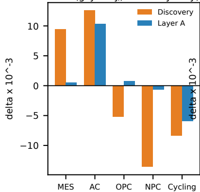
A RIG-I (grade D, Discovery-only)
