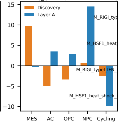
B HSF1 (grade E, cohort reversal)
