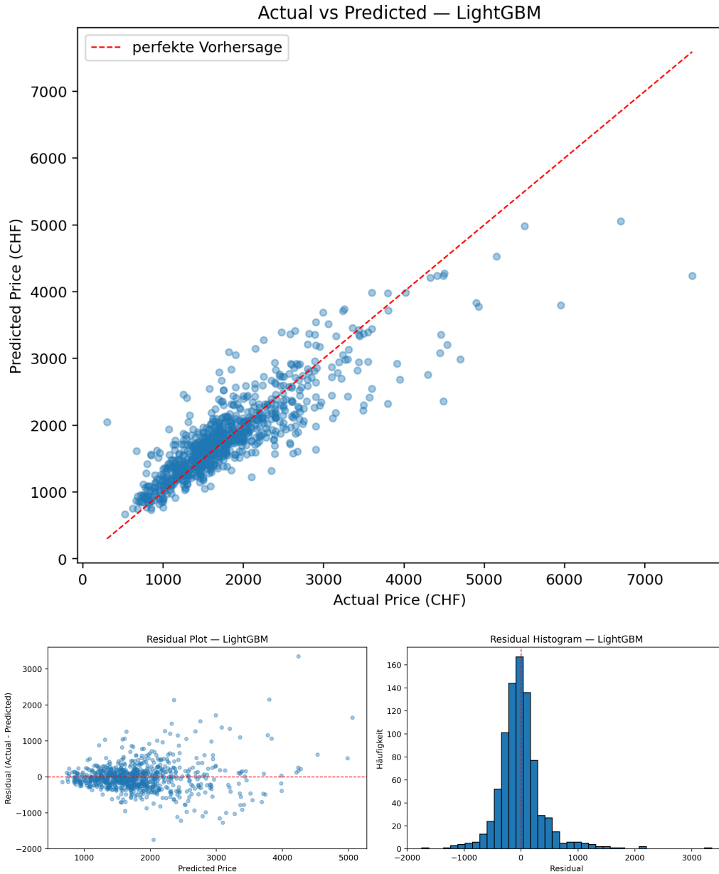
Figure 3: Actual-vs-predicted and residual analysis for the best model.
