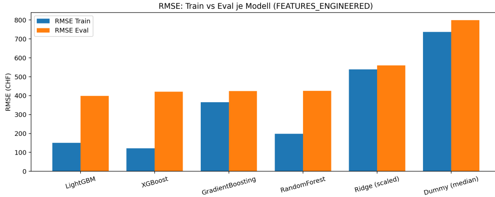
Figure 2: Train vs. Eval RMSE per model. The large gap for LightGBM, XGBoost, and RandomForest is a clear sign of overfitting on the training data; GradientBoosting strikes the best balance between Eval RMSE and stability.
