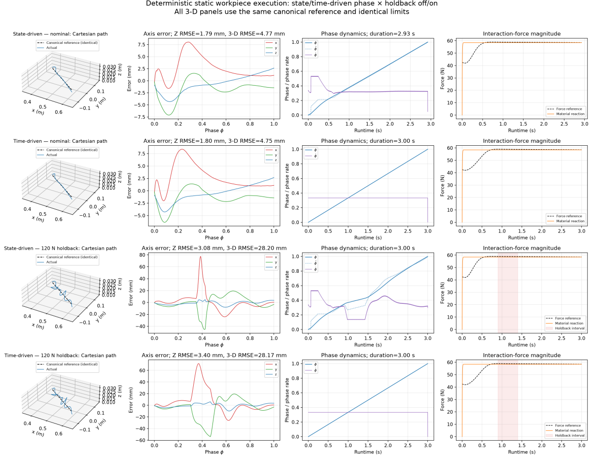
Figure 6: Deterministic static-workpiece execution without domain randomisation. Rows cross state-driven/time-driven phase with holdback disabled/enabled; columns show the Cartesian path, axis errors, phase dynamics and interaction force. Every 3-D panel uses the same canonical geometric reference and identical axis limits; only the executed trajectory changes. Nominal cut-depth RMSE is 1.795 and 1.800 mm for state- and time-driven execution, respectively. Under holdback it is 3.083 and 3.402 mm. The corresponding full Cartesian RMSE increases to 28.204 and 28.174 mm. Thus this 120 N test demonstrates constraint handling and phase response under a severe disturbance, not high-accuracy rejection of that disturbance.
