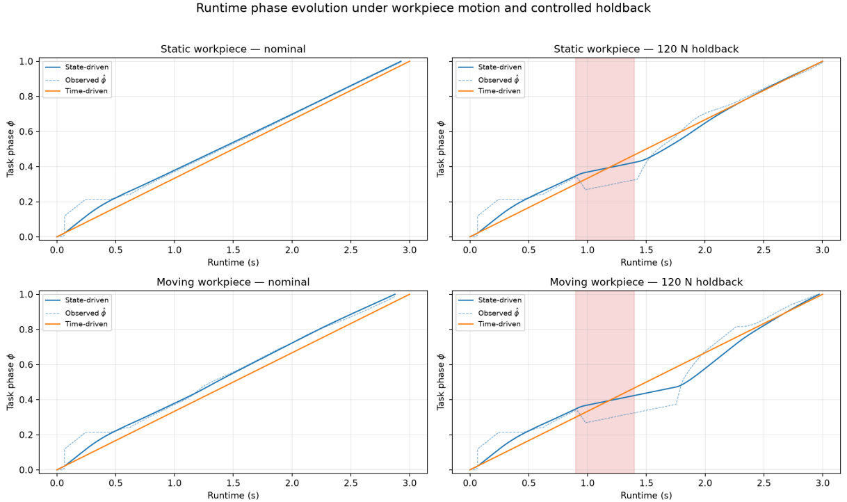
Figure 4: Representative runtime phase evolution for static and moving workpieces, with and without the controlled holdback. The red interval is the physical perturbation (63). In nominal runs the two laws remain close. Under holdback, the measured projection \hat{\phi} falls behind the commanded phase and the state-driven law retards progress, whereas the time-driven phase continues at its clock rate.
