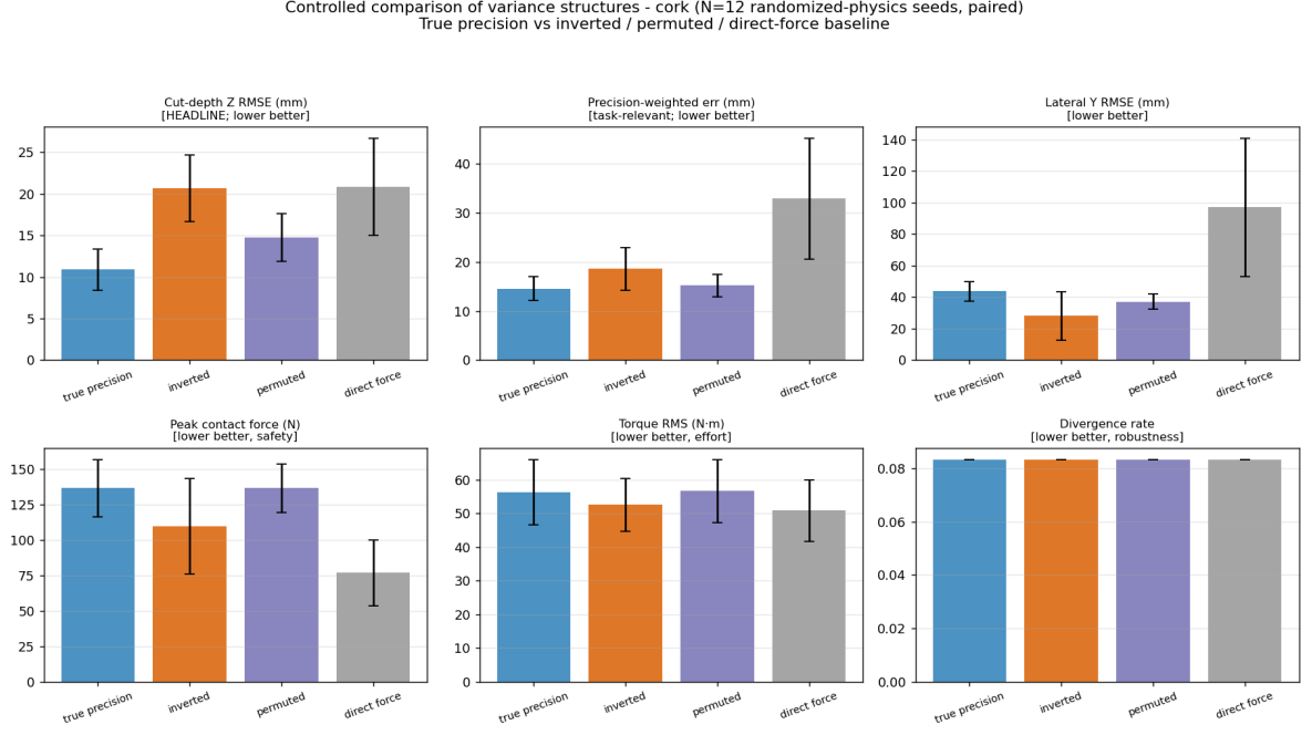
Figure 3: Controlled comparison of gain assignments on cork ( N_{\text{seed}} = 12 randomised-physics seeds, paired). Only the identified precision attains low cut-depth error; inverting or permuting the learned structure degrades it. Bars denote mean \pm std.
