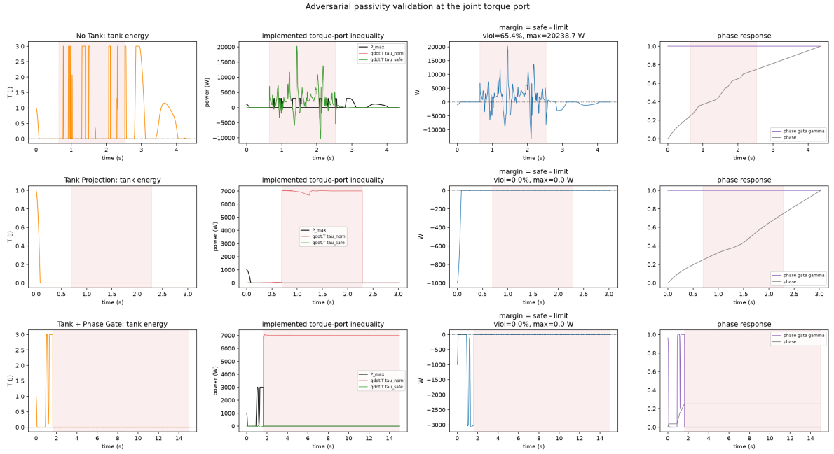
Figure 8: Positive-power perturbation validation on cork. A known positive joint-power burst is injected before the torque projection. Without projection (top row), \dot{q}^\top \tau exceeds the counterfactual budget for 65.4% of samples and reaches a maximum margin of +20,239 W. With torque projection (middle and bottom), the implemented inequality \dot{q}^\top \tau_{\text{safe}} - P_{\text{max}} \leq 0 has 0.0% logged violations. With the deliberately small 1 J validation tank, phase gating stops progress at \phi = 0.25 after storage depletion; safety intervention therefore does not imply task completion.
