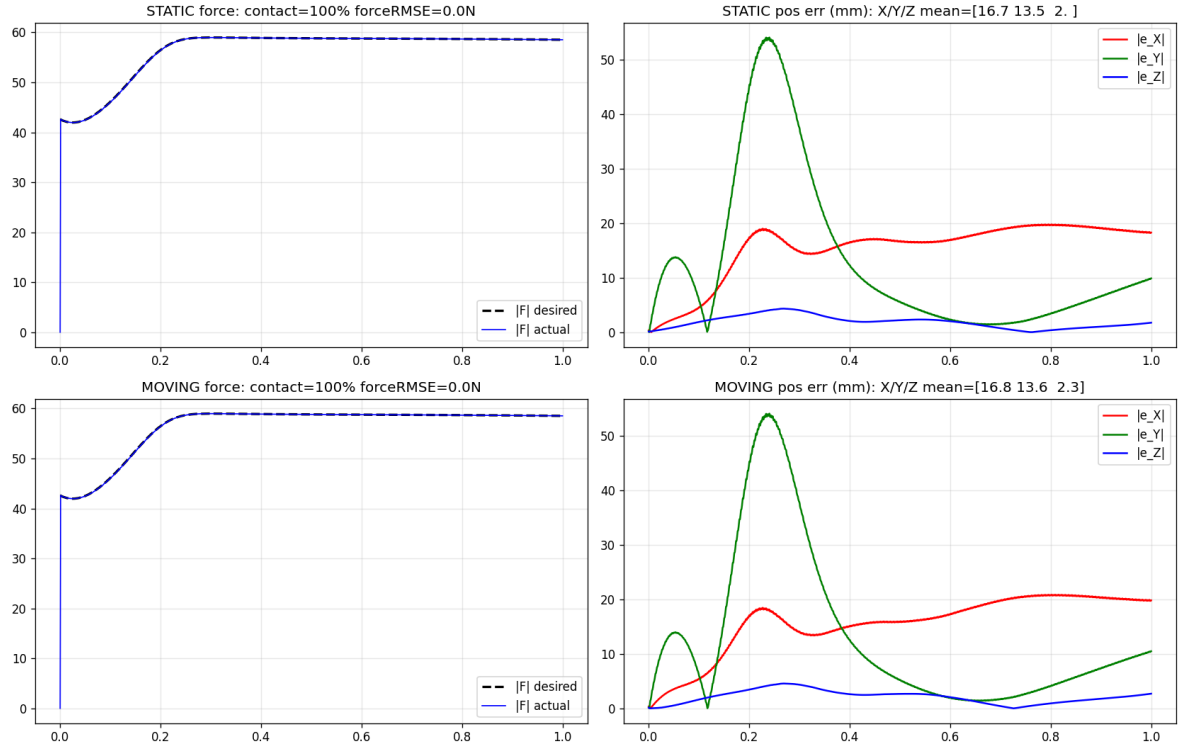
Figure 11: Cutting with the identified material model on cork . Left column: the measured contact-force magnitude (blue) follows the desired (dashed) for the whole cut, on static (top) and moving (bottom) workpieces. Right column: per-axis position error — the cut-depth (Z) error stays \approx 2 mm; the lateral (Y) error peaks during the large demonstrated lateral swing.
