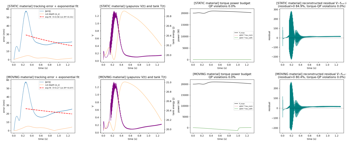
Figure 9: Nominal stability and passivity diagnostics on cork. The left column shows tracking error and cut-depth error; the middle column shows the Lyapunov diagnostic and tank energy; the third column shows the implemented torque power budget P_{\text{max}} together with nominal and projected torque power; the right column shows the reconstructed Cartesian residual, used as a diagnostic rather than as the primary passivity proof.
