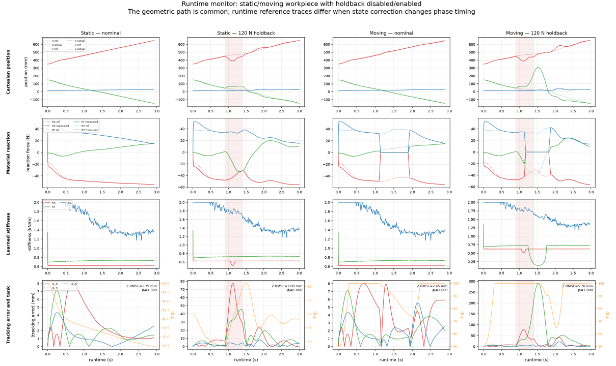
Figure 13: Runtime monitor reconstructed from four state-driven cork episodes: static nominal, static with 120 N holdback, moving nominal, and moving with holdback (columns from left to right). Rows show Cartesian position, axis-resolved material reaction, learned stiffness, and absolute tracking error with tank energy. Red shading identifies the validation-force interval [0.9, 1.4] s; the plotted reaction channel remains the identified material reaction and does not re-label the separately applied holdback as contact force. The desired world-frame path is common to all columns, although its time-indexed samples differ when state-driven phase timing changes. Representative cut-depth RMSE is 1.795, 3.083, 2.450 and 5.700 mm, respectively. The holdback columns exhibit large Cartesian displacement and must be interpreted as stress tests rather than precision-tracking results.
