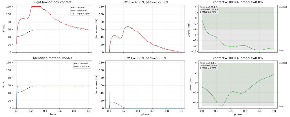
Material-model comparison: same controller, different contact physics
