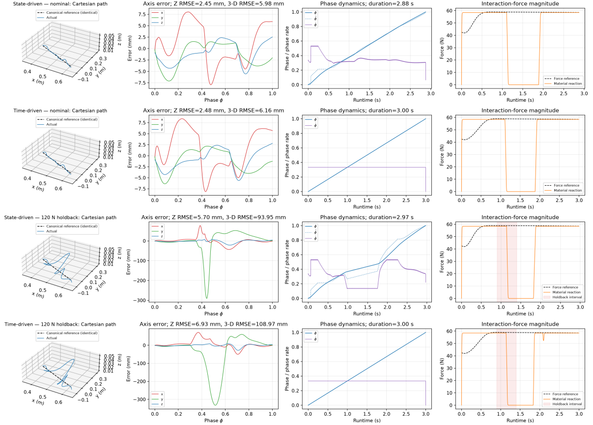
Deterministic moving workpiece execution: state/time-driven phase x holdback off/on All 3-D panels use the same canonical reference and identical limits
