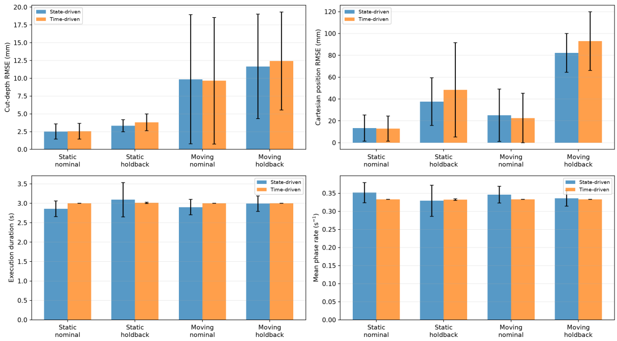
Figure 5: Performance over the complete factorial study. Error bars show one standard deviation across paired randomised-physics seeds. State-dependent timing trades execution time for synchronisation when measured progress lags; its rate can also exceed the clock rate when the state projection is ahead.
