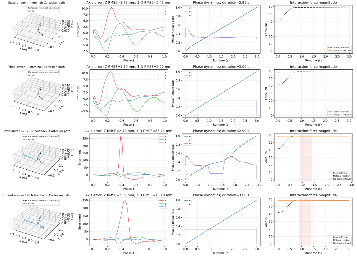
Figure 6: Deterministic static-workpiece execution without domain randomisation. Rows cross state-driven/time-driven phase with holdback disabled/enabled; columns show the Cartesian path, axis errors, phase dynamics and interaction force. Every 3-D panel uses the same canonical geometric reference and identical axis limits; only the executed trajectory changes. Nominal cut-depth RMSE is 1.776 and 1.791 mm for state- and time-driven execution, respectively. Under holdback it is 2.424 and 2.393 mm. The corresponding full Cartesian RMSE increases to 83.208 and 76.179 mm. Thus this 120 N test demonstrates constraint handling and phase response under a severe disturbance, not high-accuracy rejection of that disturbance.
