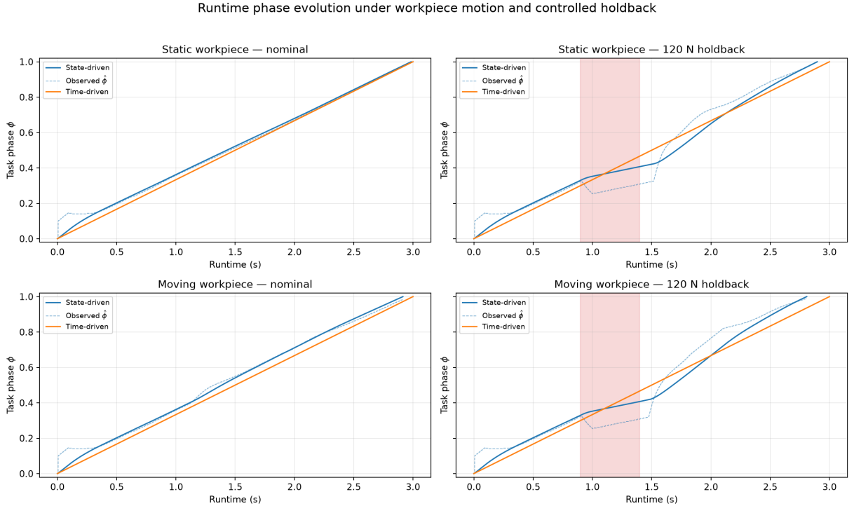
Figure 4: Representative runtime phase evolution for static and moving workpieces, with and without the controlled holdback. The red interval is the physical perturbation (62). In nominal runs the two laws remain close. Under holdback, the measured projection \hat{\phi} falls behind the commanded phase and the state-driven law retards progress, whereas the time-driven phase continues at its clock rate.
