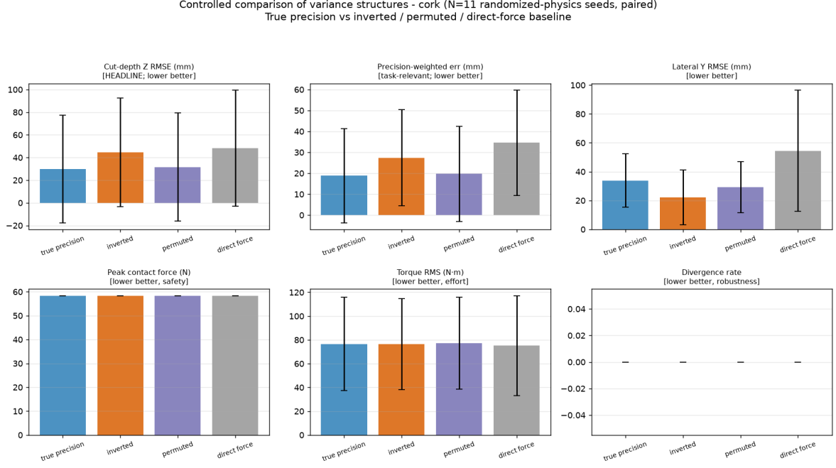
Figure 3: Controlled comparison of gain assignments on cork ( N_{\text{seed}} = 11 randomised-physics seeds, paired). Only the identified precision attains low cut-depth error; inverting or permuting the learned structure degrades it. Bars denote mean \pm std.
