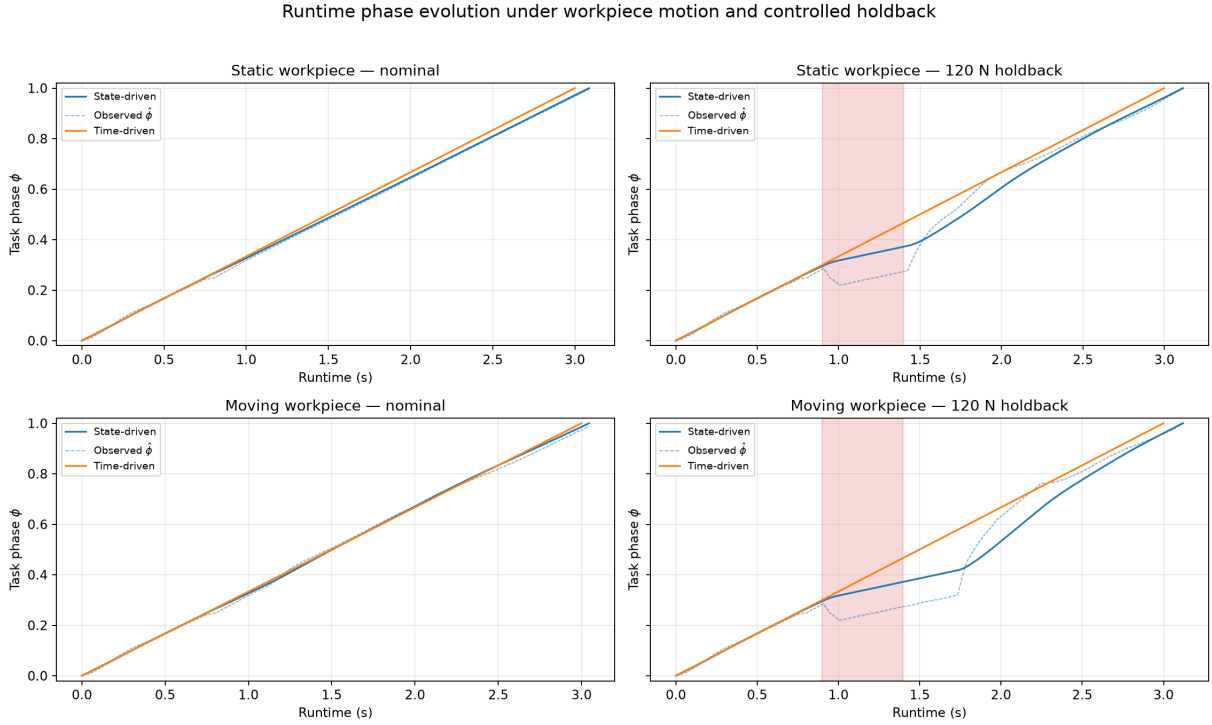
Figure 4: Representative runtime phase evolution for static and moving workpieces, with and without the controlled holdback. The red interval is the physical perturbation (64). In nominal runs the two laws remain close. Under holdback, the measured projection \hat{\phi} falls behind the commanded phase and the state-driven law retards progress, whereas the time-driven phase continues at its clock rate.
