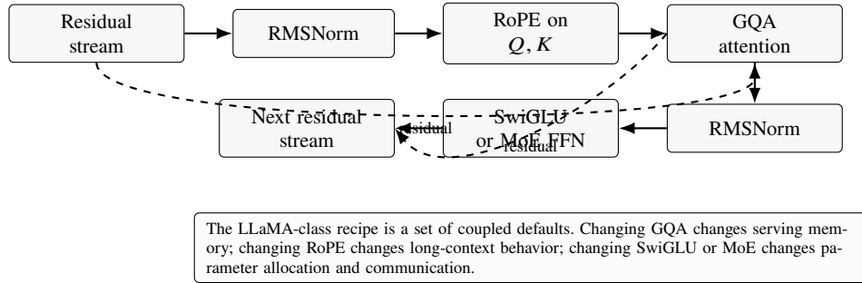
Fig. 5.1 A LLaMA-class decoder block as a contract among normalization, position handling, attention cache structure, and feed-forward capacity. The drawing abstracts from LLaMA, Llama 2/3, DeepSeek-V3, and Kimi K2-style reports without copying any released architecture figure.
