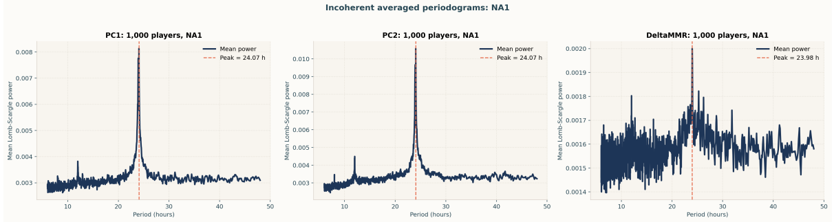
Figure 1: Incoherently averaged within-subject Lomb–Scargle periodograms for one server (NA1, 1,000 players). PC1 (left) and PC2 (centre) show sharp circadian peaks at 24.07 h; \Delta MMR (right) shows a weak, noisy spectrum with peak power roughly an order of magnitude smaller and no clear circadian component.
