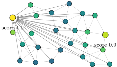
(a) global softmax: one auction
