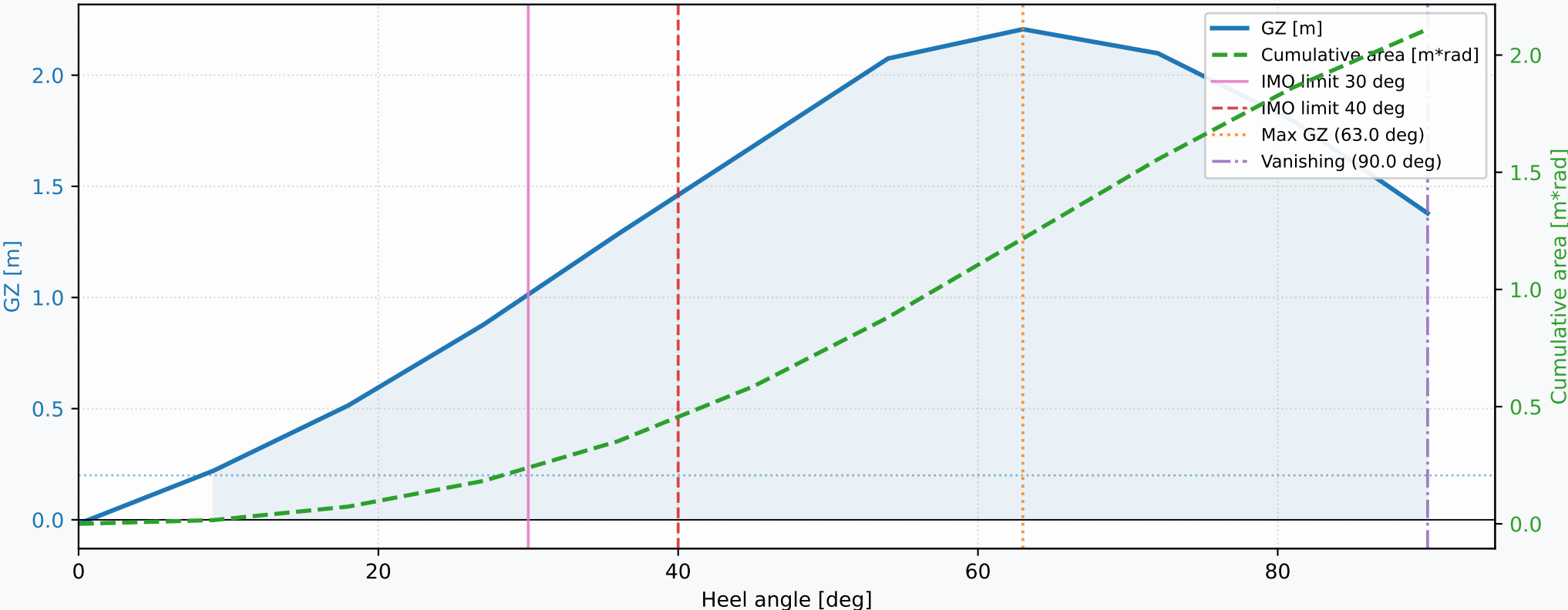
GZ Righting Lever Curve
