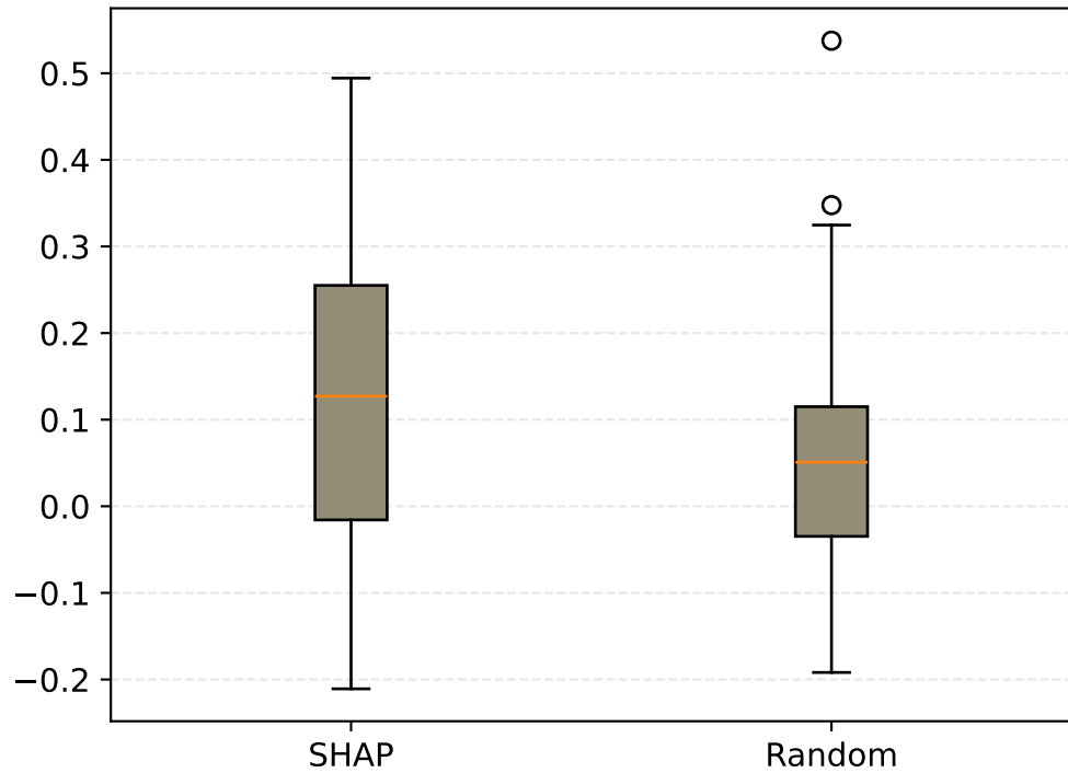
AOPC — deletion
