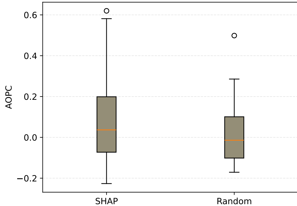
AOPC — insertion
