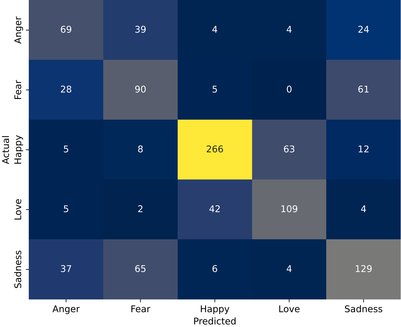
ME-XBAL confusion matrix — Tokopedia test set (n=1081, seed=42)
