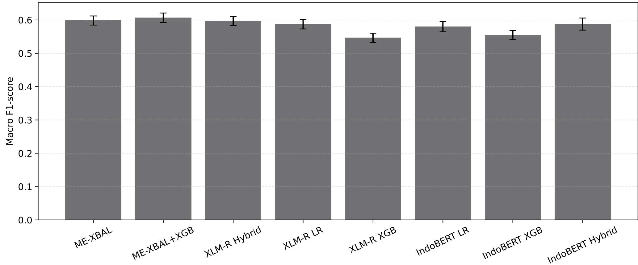
Model comparison — Tokopedia (mean \pm std over 10 seeds)
