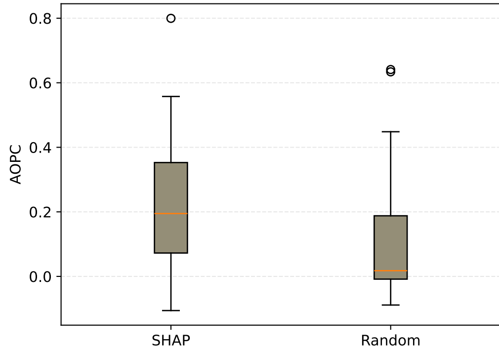
AOPC — deletion
