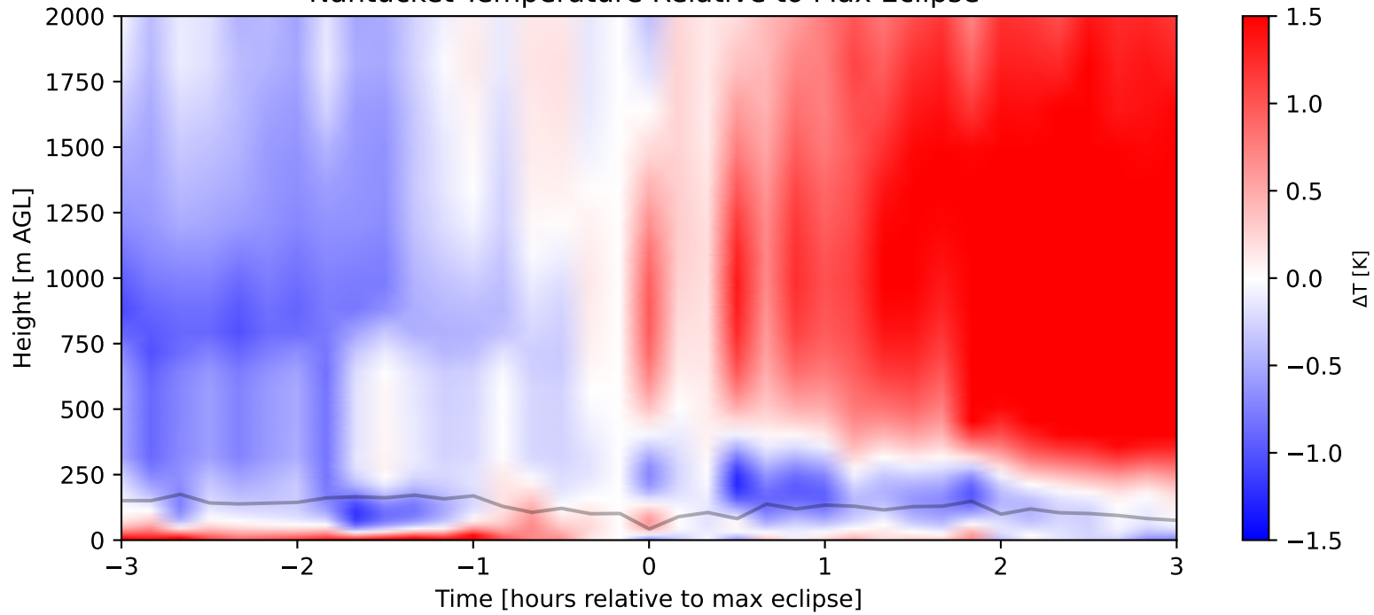
Nantucket Temperature Relative to Max Eclipse
