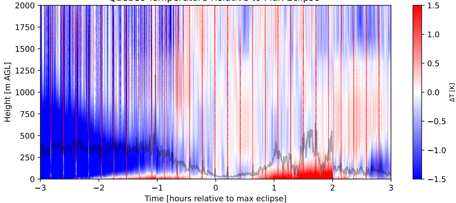
Québec Temperature Relative to Max Eclipse
