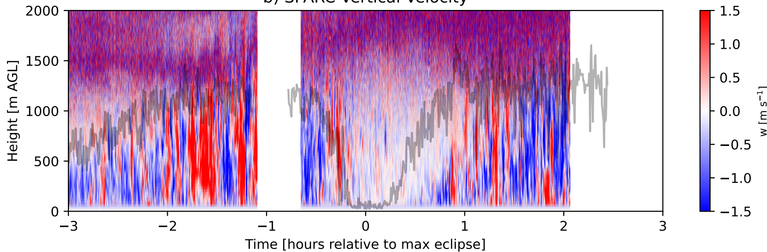
b) SPARC Vertical Velocity
