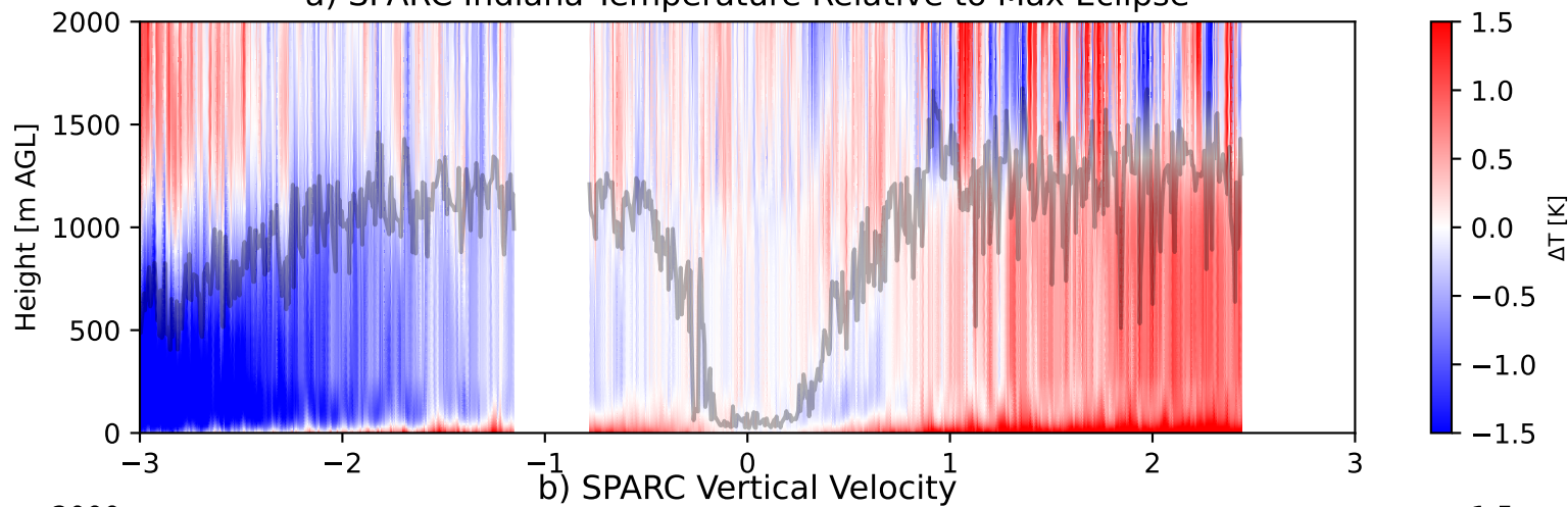
a) SPARC Indiana Temperature Relative to Max Eclipse
