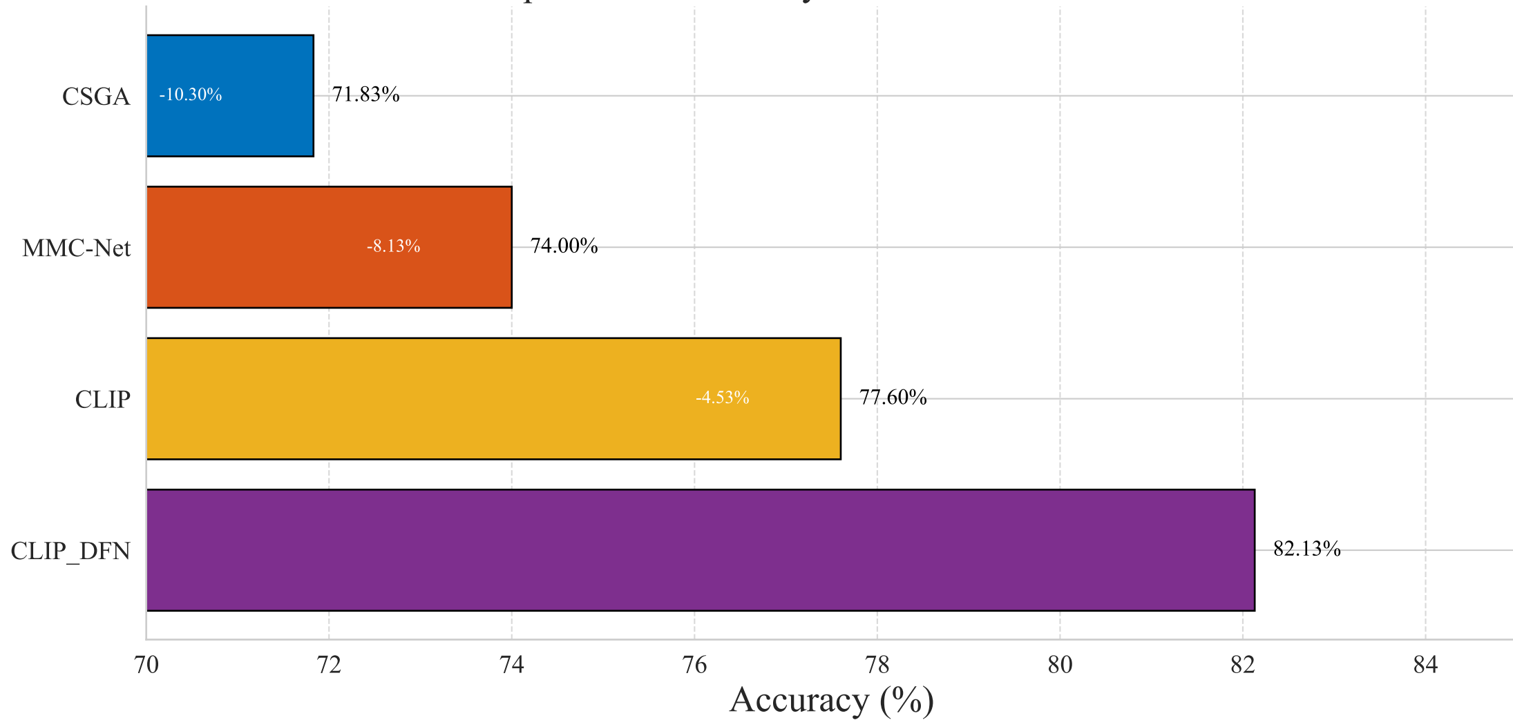
Comparison of Accuracy Across Different Methods
