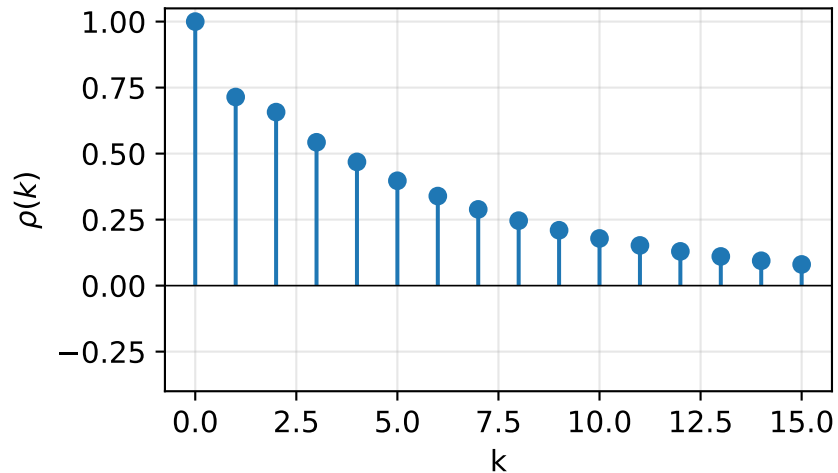
ACF AR(2) \phi_1 = 0.5, \phi_2 = 0.3
