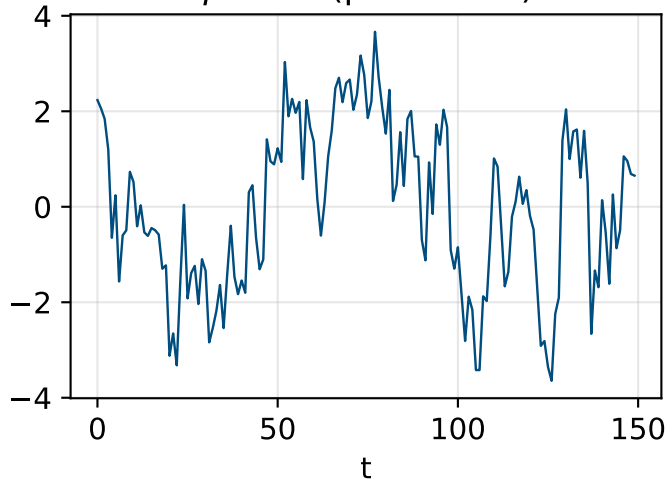
\phi = 0.8 (persistant)
