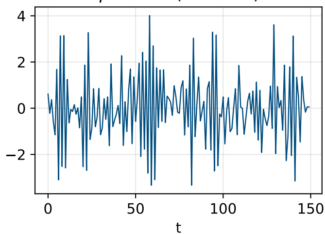
\phi = -0.8 (oscillant)
