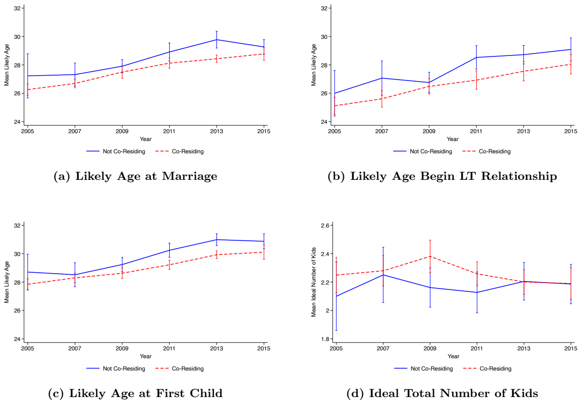
Figure 2: Average Expected Age at Family Formation Events by Co-Residence Status
