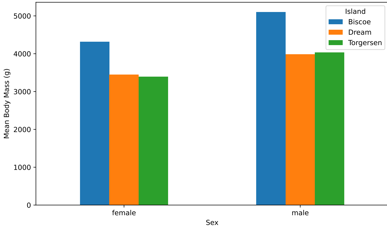
Mean Body Mass by Sex and Island (Python)
