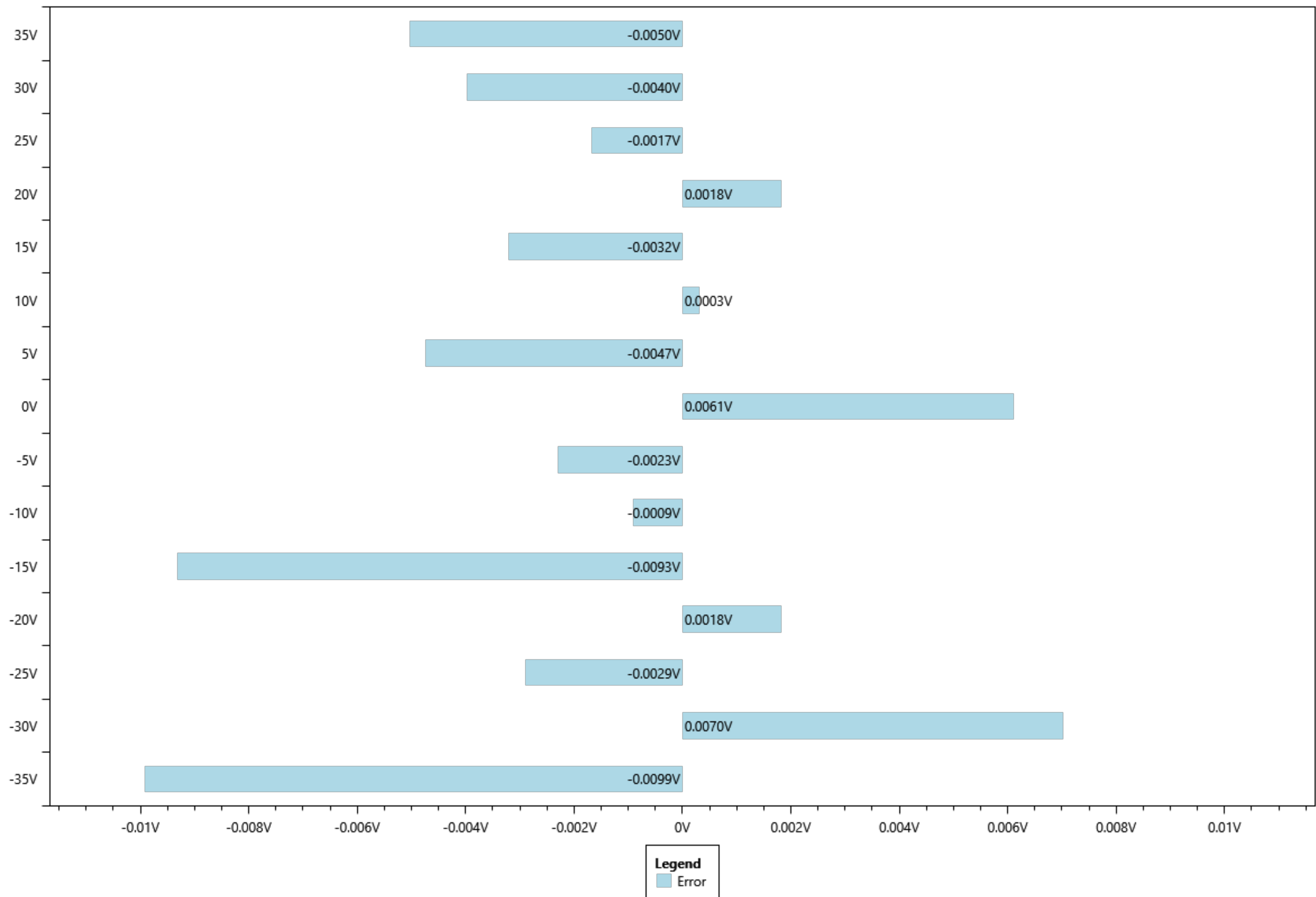
Channel 1 errors for Measurement
