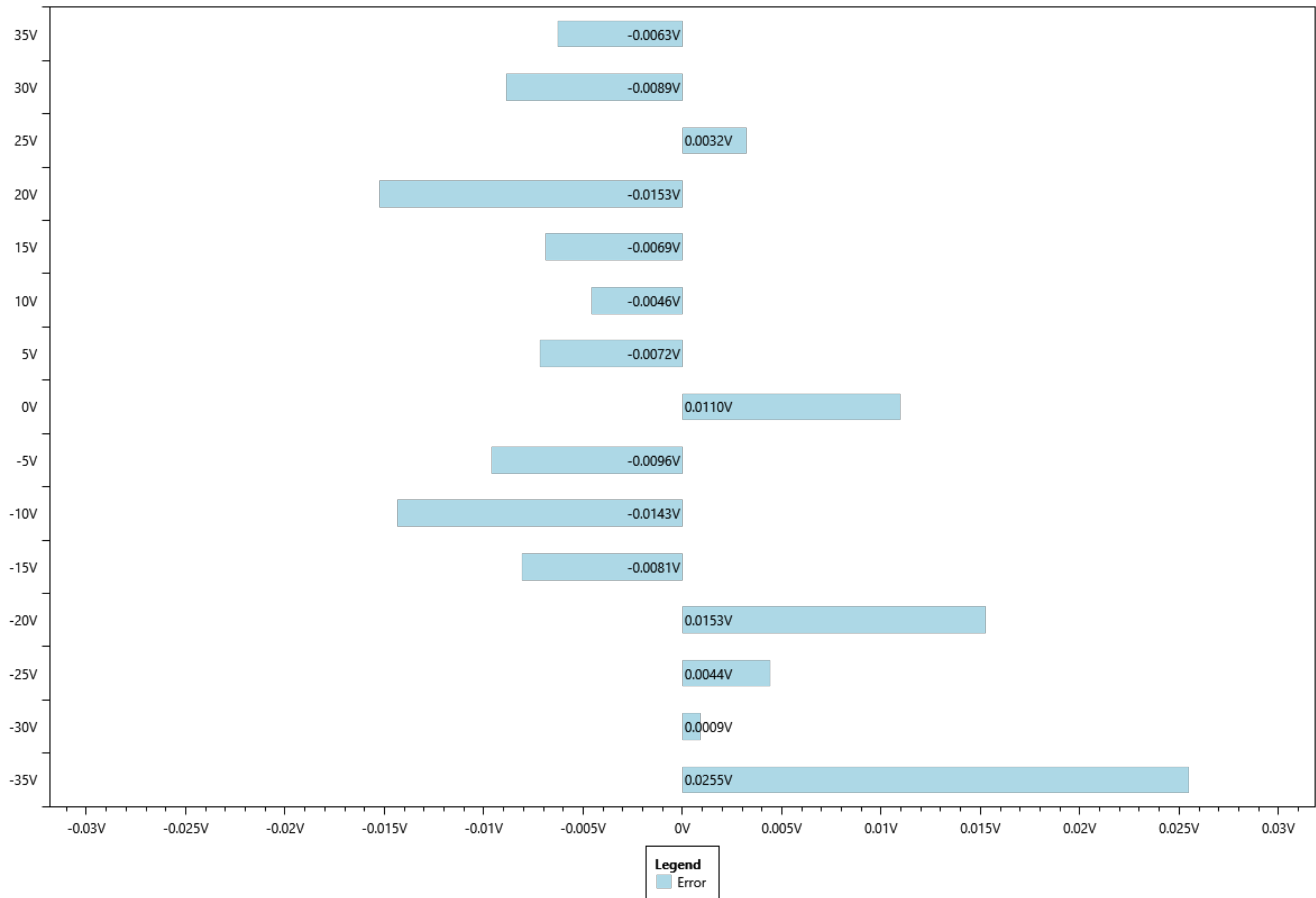
Channel 4 errors for Measurement
