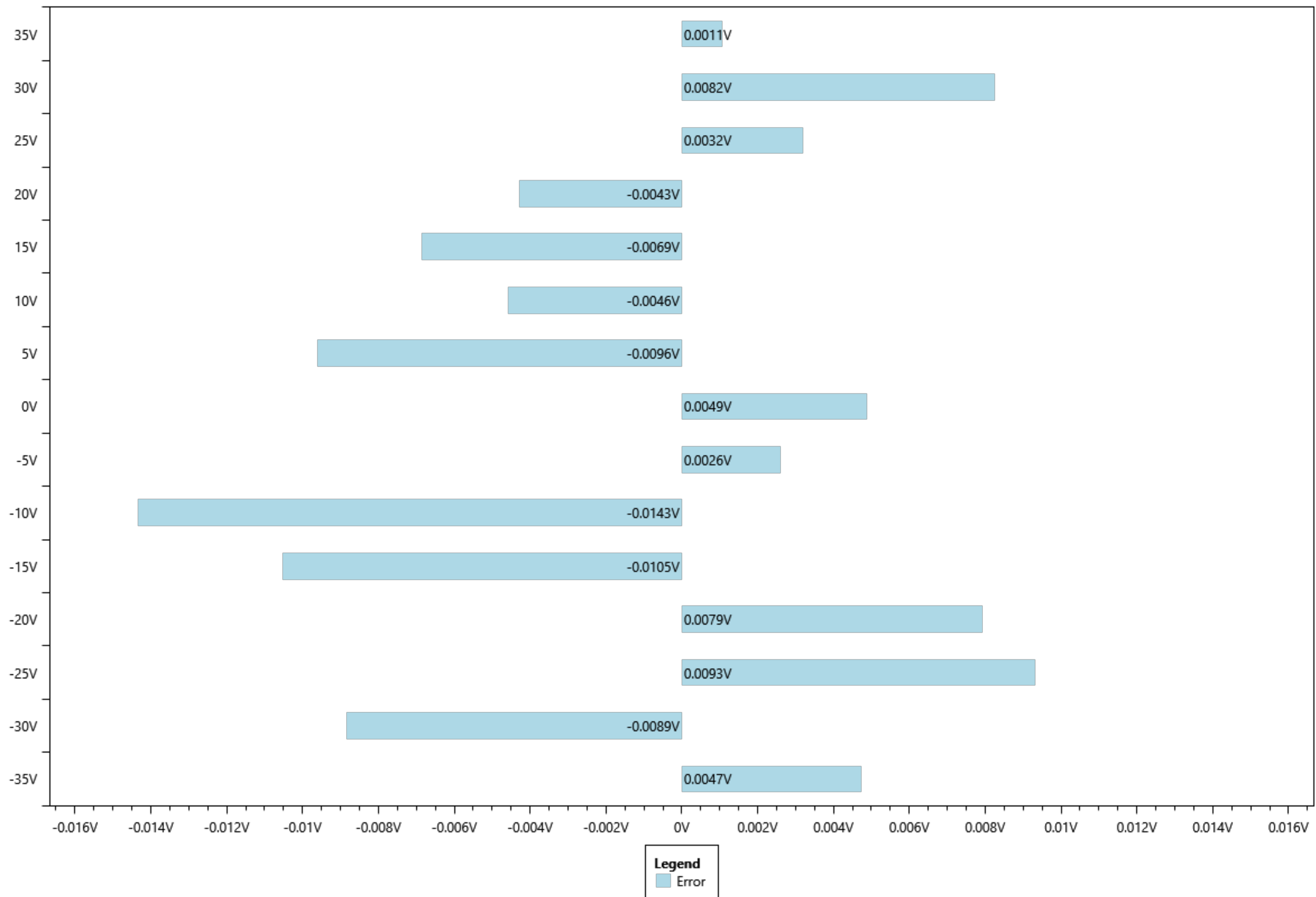
Channel 3 errors for Measurement
