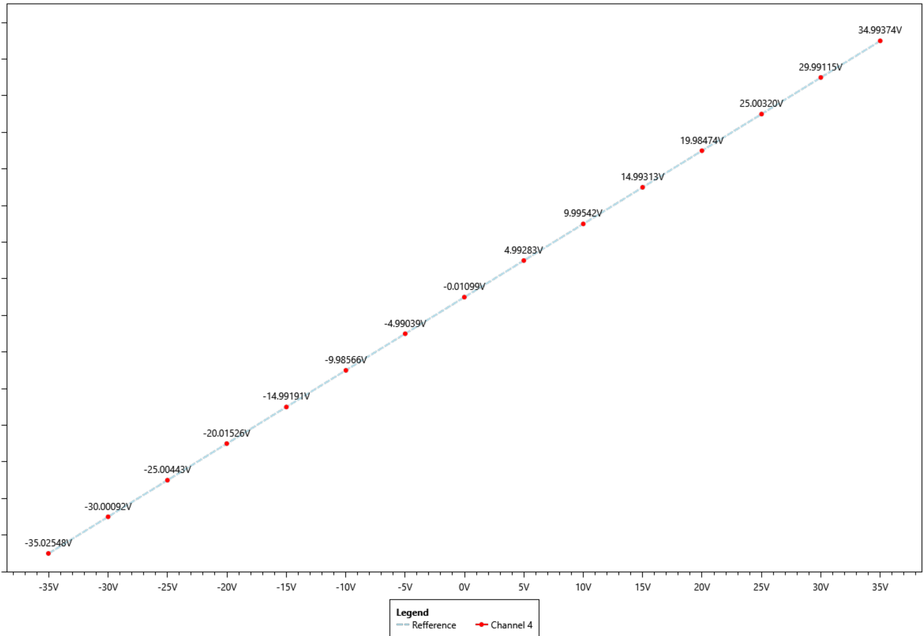
Channel 4 values for Measurement
