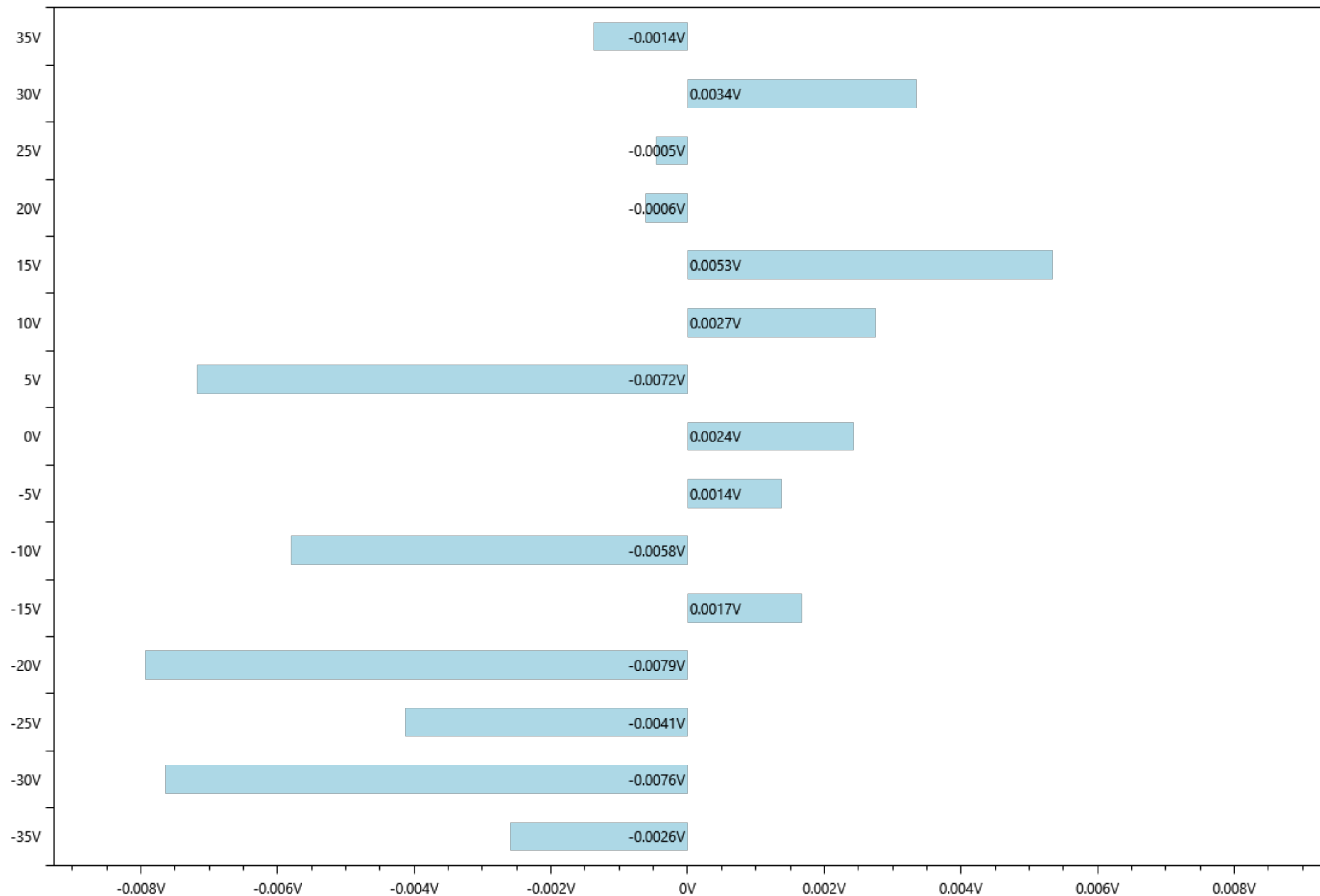
Channel 2 errors for Measurement
