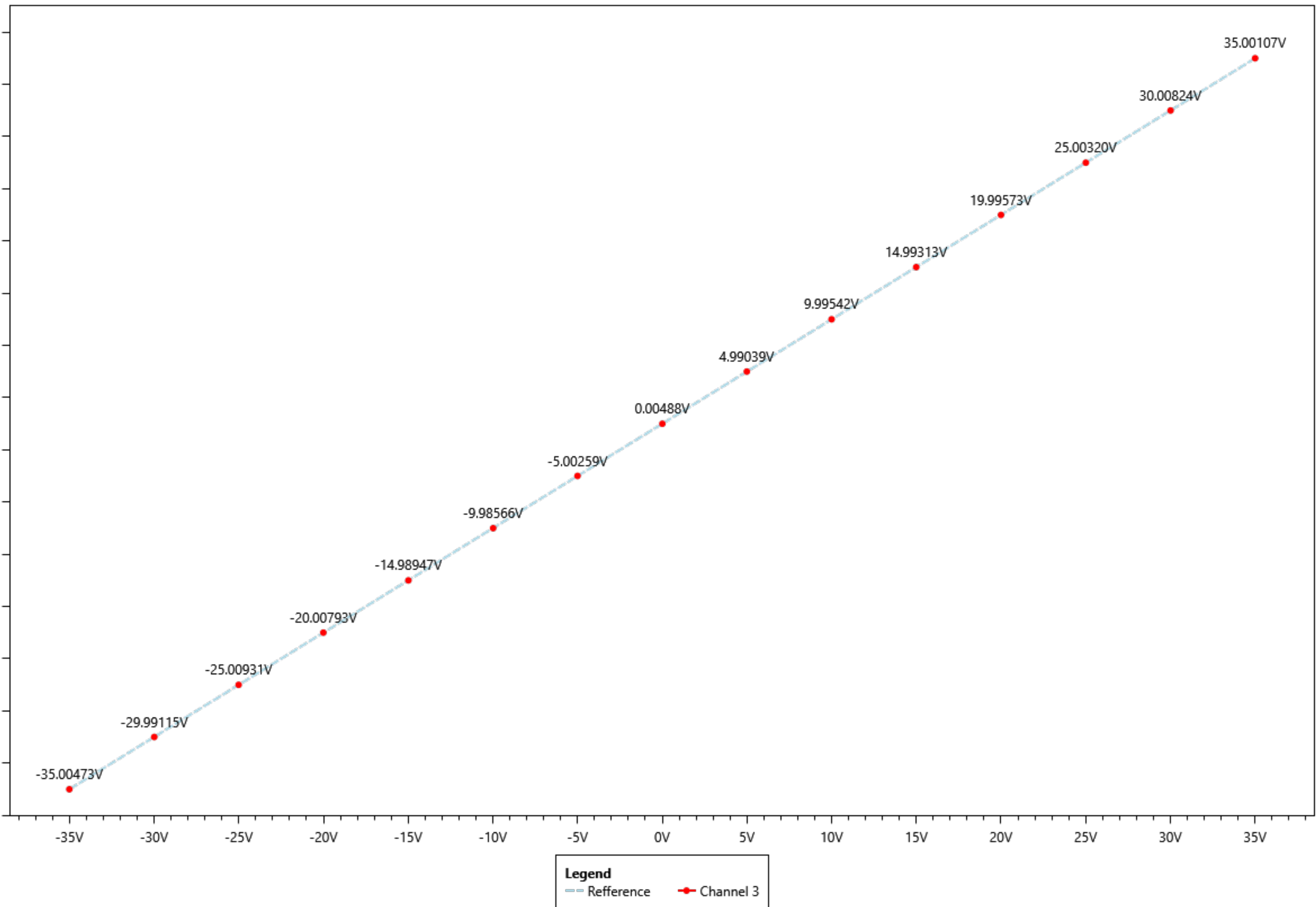
Channel 3 values for Measurement
