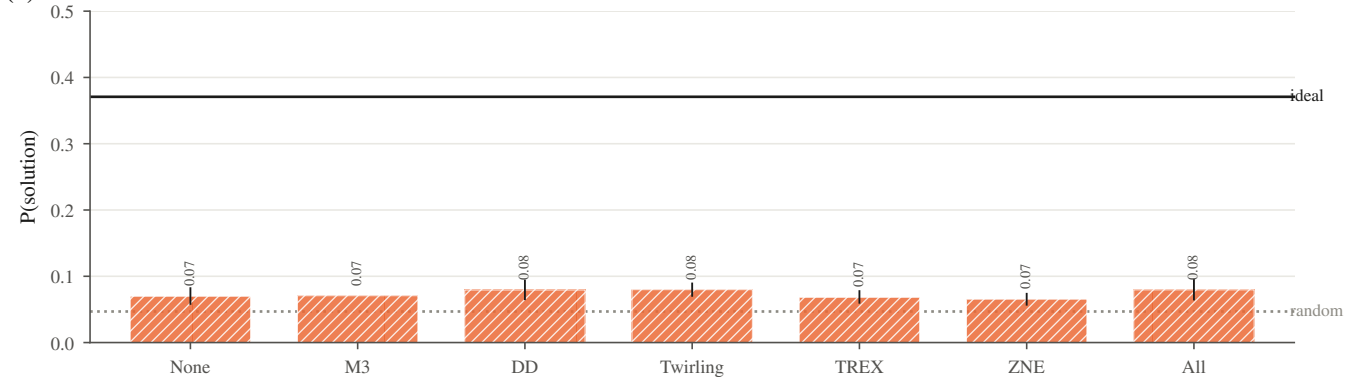
(b) 6-variable K-SAT (6 variables, 7 clauses), Oracle A, k = 1
