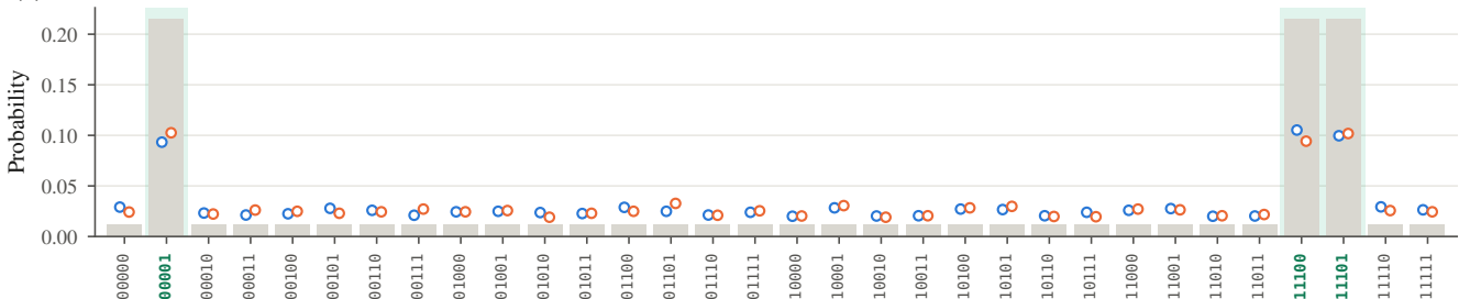
(b) 5-variable K-SAT, k = 2 (ideal P = 1.000 ); solutions shaded
