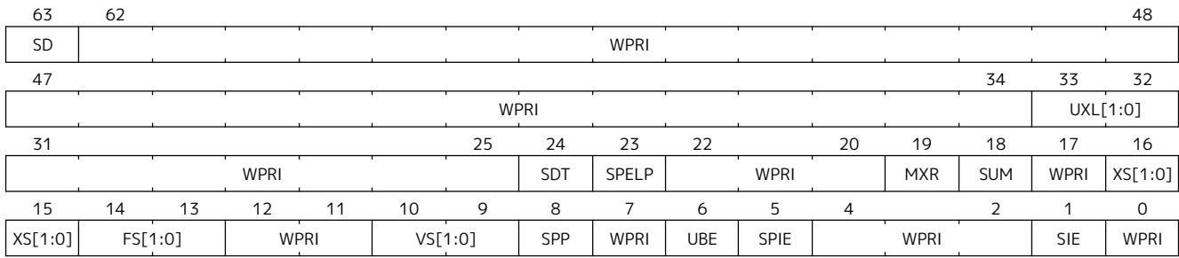
Figure 92. Virtual supervisor status ( vsstatus ) register when VSXLEN =64.
