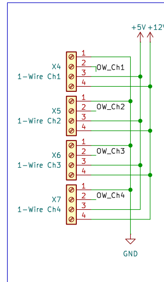
1-Wire Terminals
