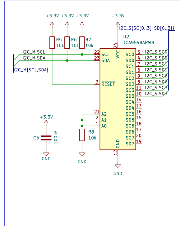
I2C Multiplexer
