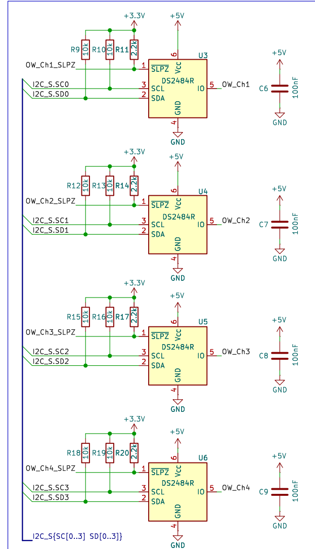
1-Wire Busmaster
