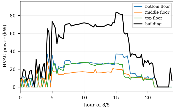
AIF (fixed ref.) (peak 83.8 kW)
