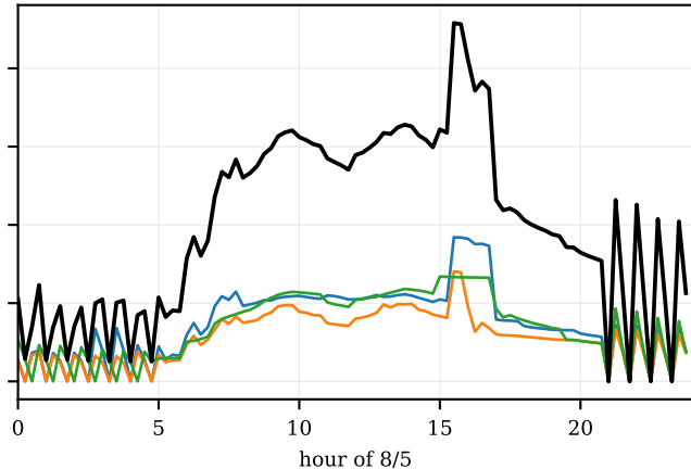
RBC proactive (peak 91.6 kW)
