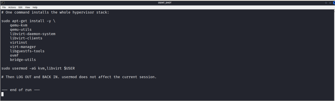
Screenshot: the single hypervisor install command and the group membership step.
