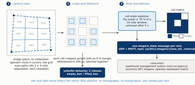
Figure 3. The rack-cell path: a 3 × 3 operator-drawn grid, batched per-cell classification, and one retained state message per rack.
