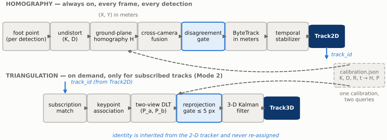
Figure 3. The geometric pipeline: always-on homography chain (foot point → undistortion → H → fusion → disagreement gate → ByteTrack-in-meters → stabilizer → Track2D) and subscription-driven triangulation branch (association → two-view DLT → reprojection gate → 3D Kalman → Track3D); shared calibration and identity space highlighted.
