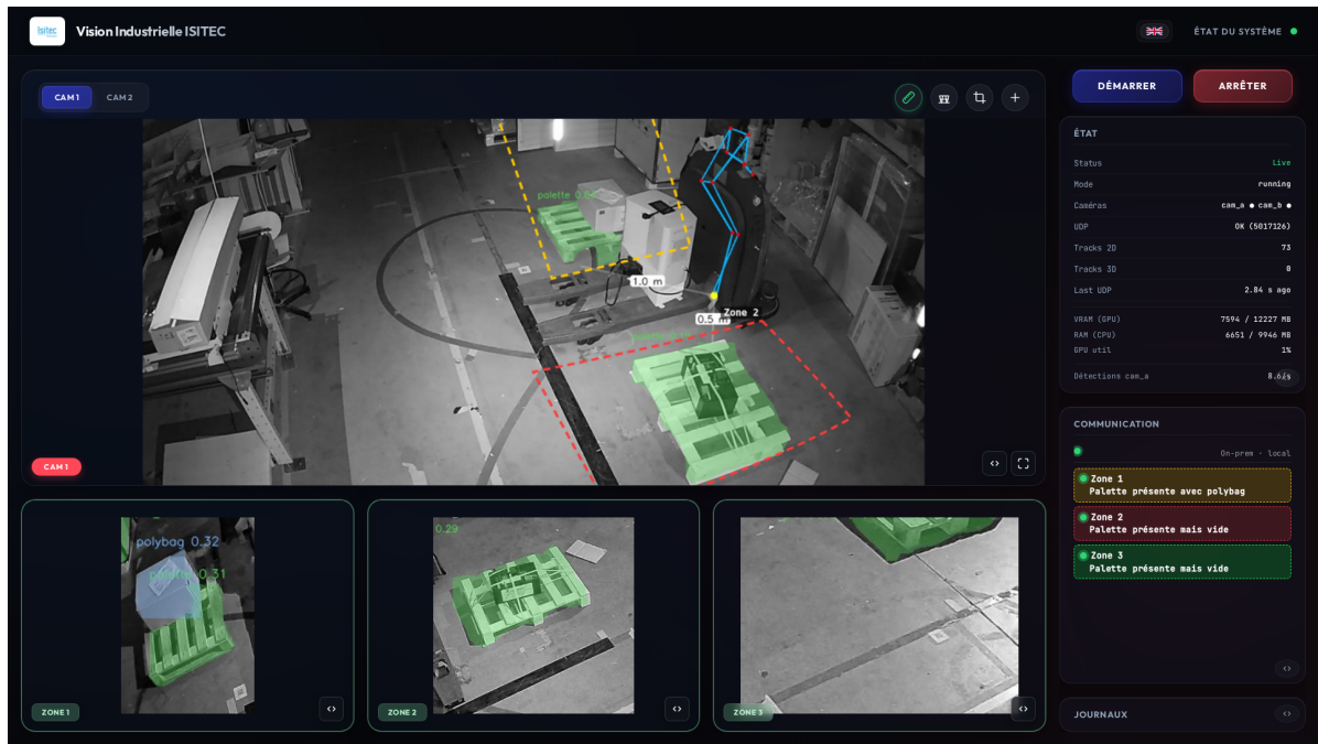
Figure 6. The operator dashboard during the measured production run — live camera view with instance-segmented pallets, configured zone polygons, a tracked person with pose skeleton and metric proximity distances (1.0 m / 0.5 m to a zone), per-zone occupancy cards driven by the MQTT zone-state stream, and the runtime status panel (dual-camera Live, Track2D count, UDP counters, GPU memory).
