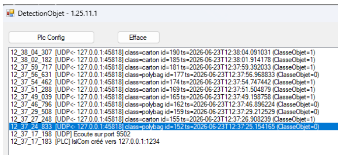
Figure 10. Datagram detail in the customer's receiver: per-parcel class, track id, timestamp, and the ClasseObjet flag read by the PLC.
