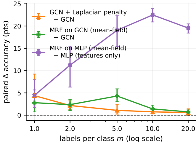
(b) Benefit of the prior, paired by seed
