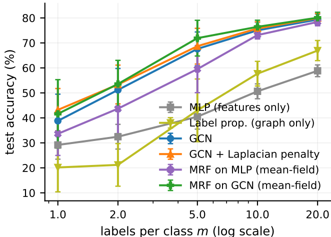
(a) Cora: accuracy vs. label budget
