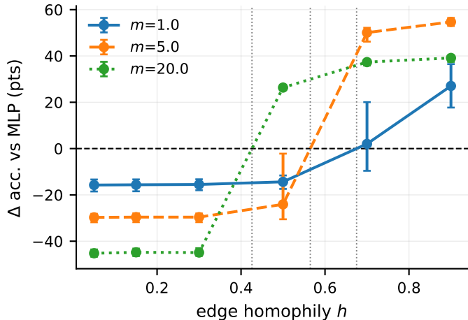
(a) Dogmatic prior: benefit and harm
