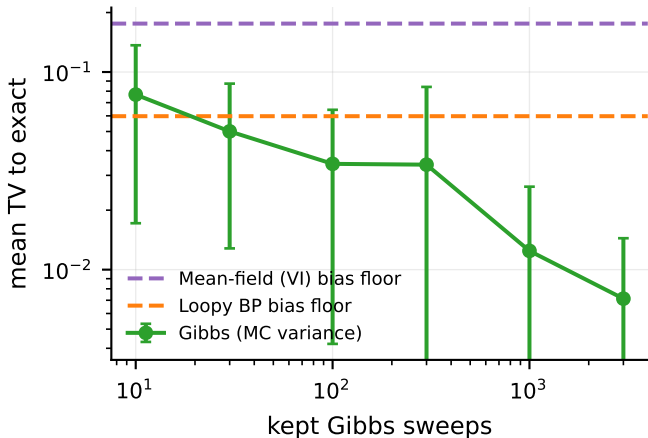
Bias vs variance (4x4 grid, \beta=1.75 )
