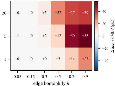
(b) tuned prior ( \beta chosen on validation)
