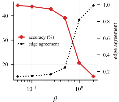
(c) CSBM h=0.05 : collapse
