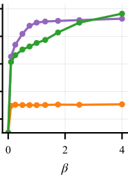
star (hub tree)
