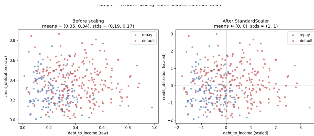
Figure 5. Before vs after StandardScaler : same shape, different location and scale.
