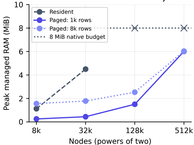
Crosses: resident allocation rejected
