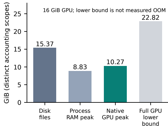
(b) 1B-edge storage footprint
