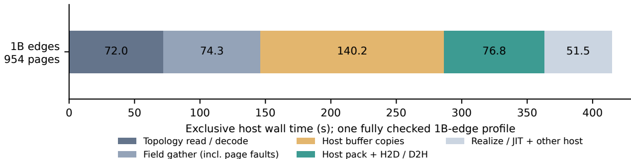
(c) 1B-edge execution cost: 414.81 s
