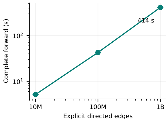
(a) Capacity through 1B edges
