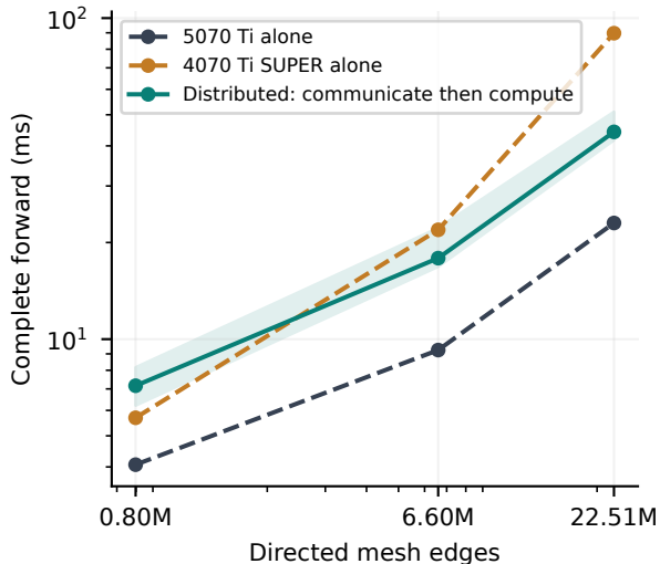
(a) Spatial-mesh distributed execution
