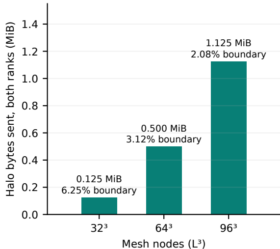
(b) Halo grows with interface area
