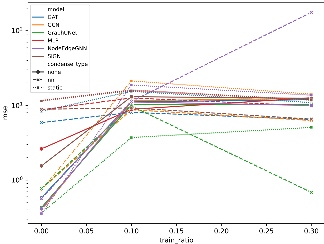
test on rectangle_sin2_left+right with characteristic length 0.1
