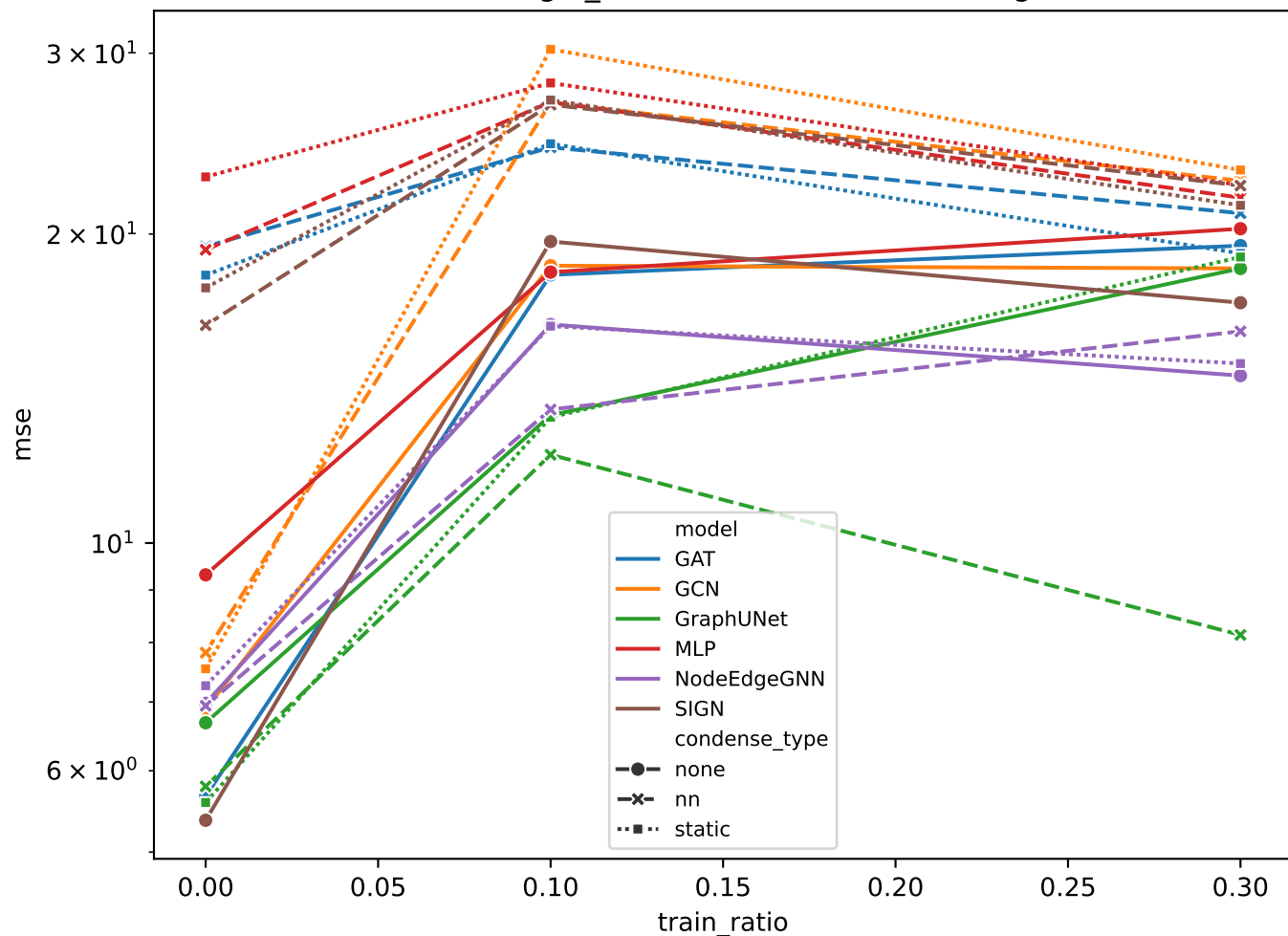
test on rectangle_sin1 with characteristic length 0.1
