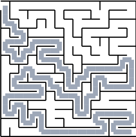
Puzzle 2
