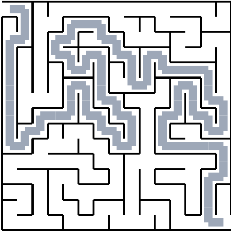
Puzzle 5
