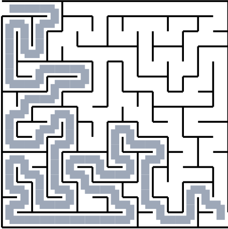
Puzzle 3
