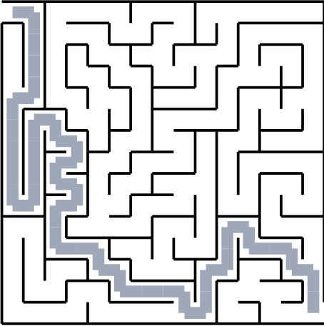
Puzzle 4
