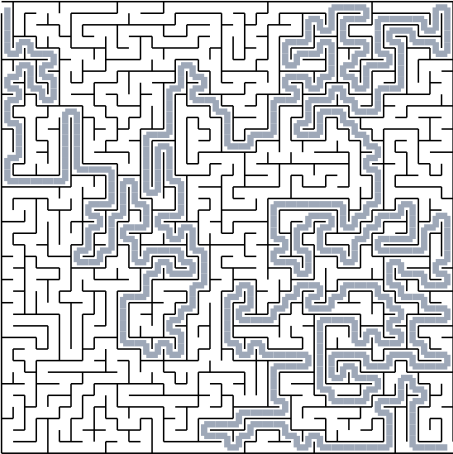
Puzzle 20
