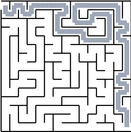
Puzzle 1
