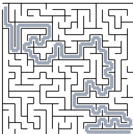
Puzzle 16
