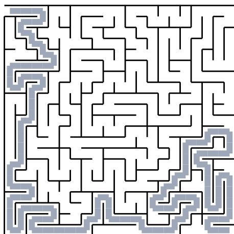
Puzzle 18
