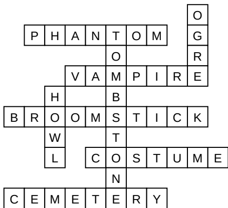
Puzzle 3
