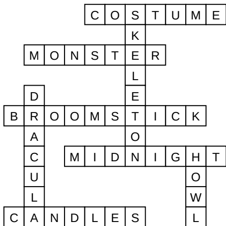
Puzzle 5
