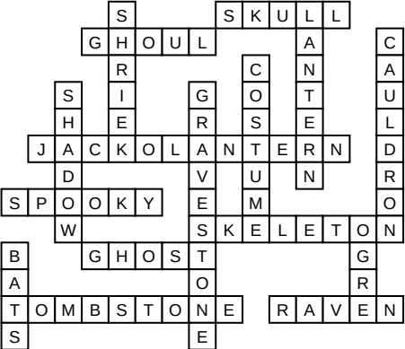
Puzzle 12
