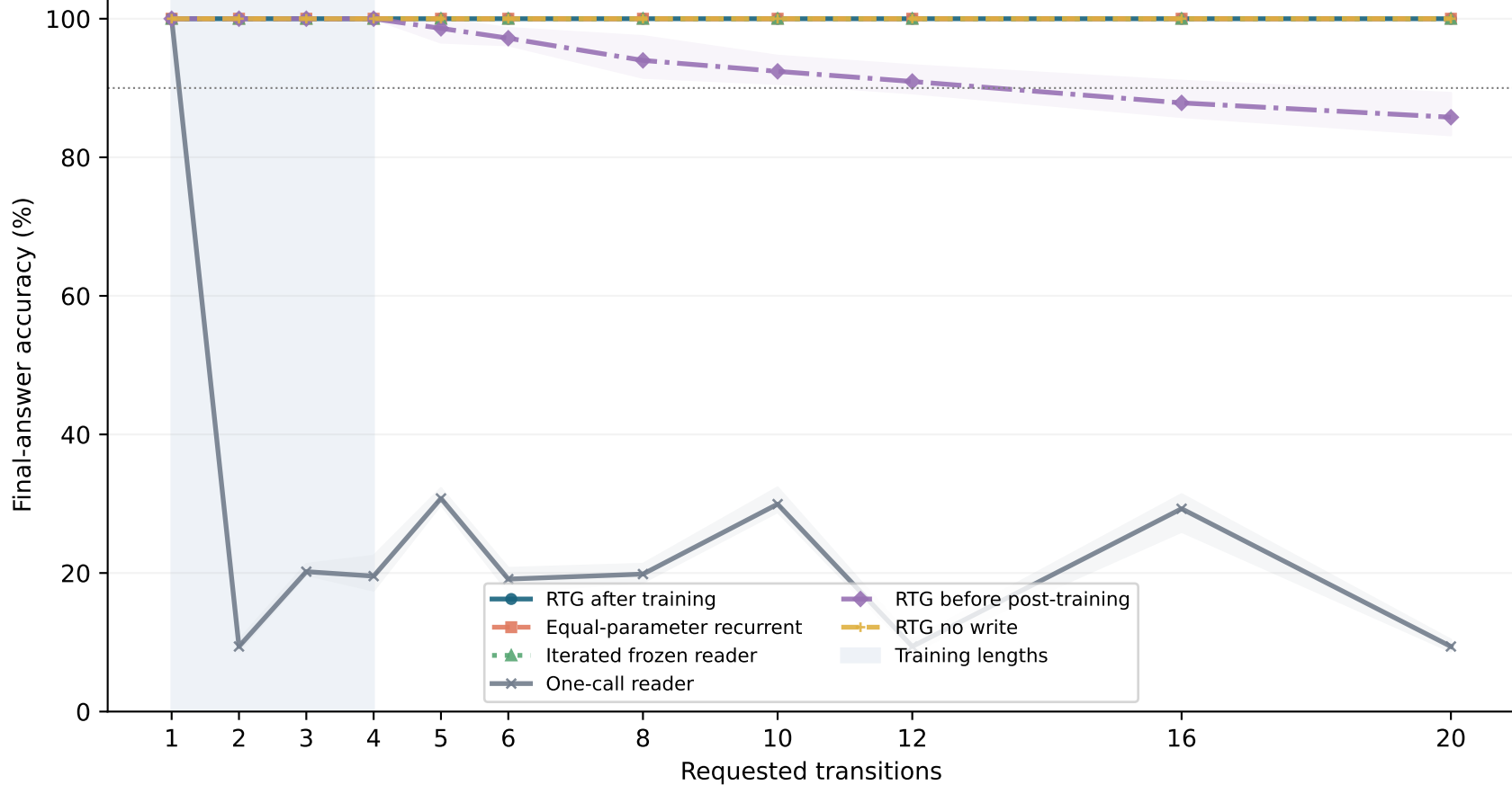
Phase A: static rule composition on unseen permutations
