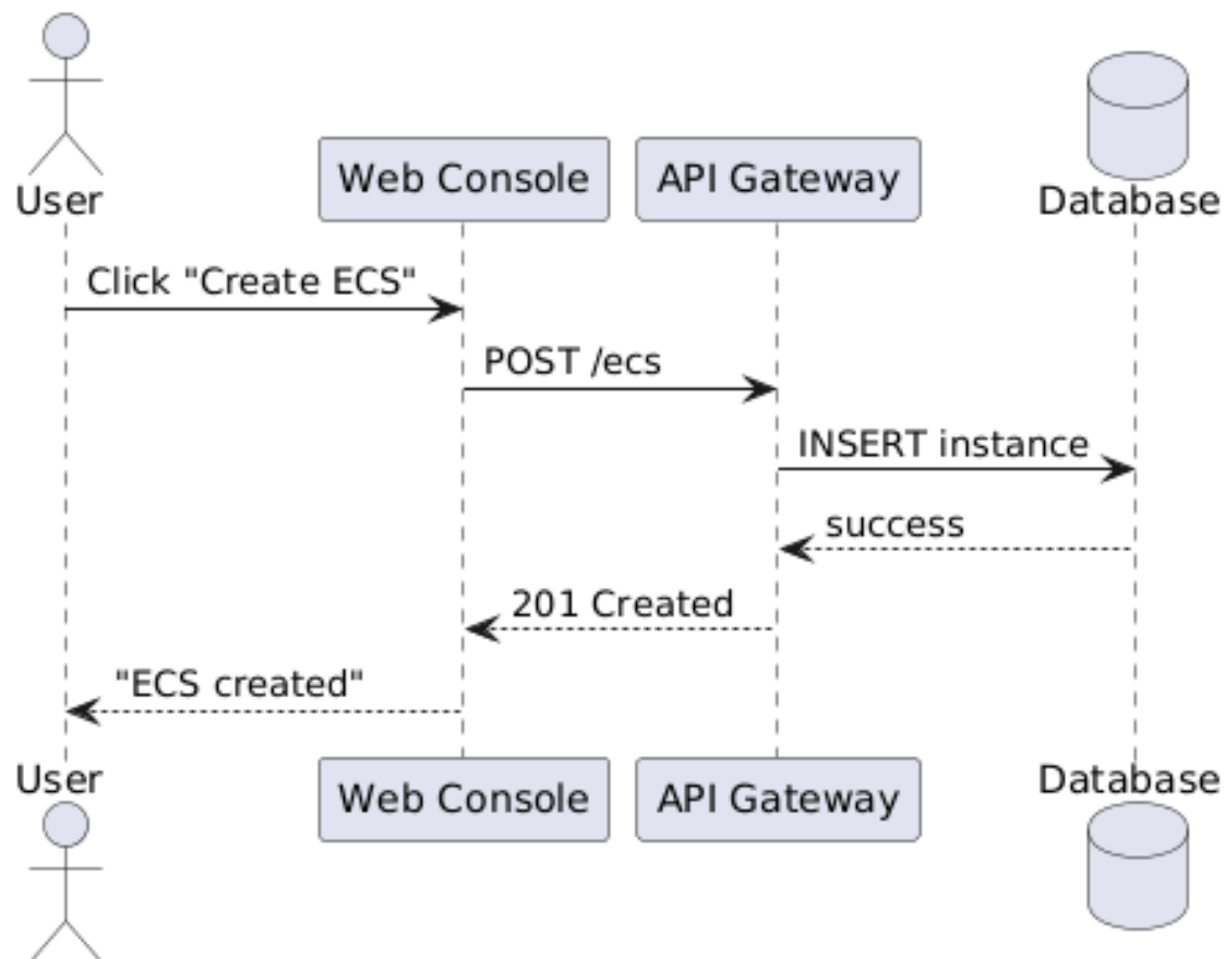
Diagram 1: Sequence diagram of ECS creation
