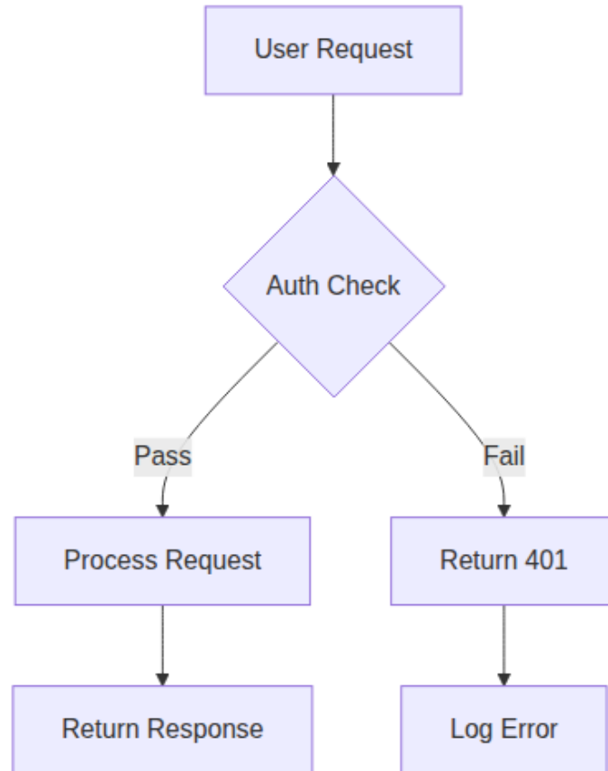
Diagram 3: Flowchart of request authentication
